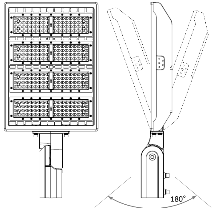
Slip-Fitter Mount LEDMPALPRO-SF
