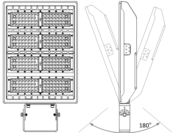
Trunnion Mount LEDMPALPRO-TR
