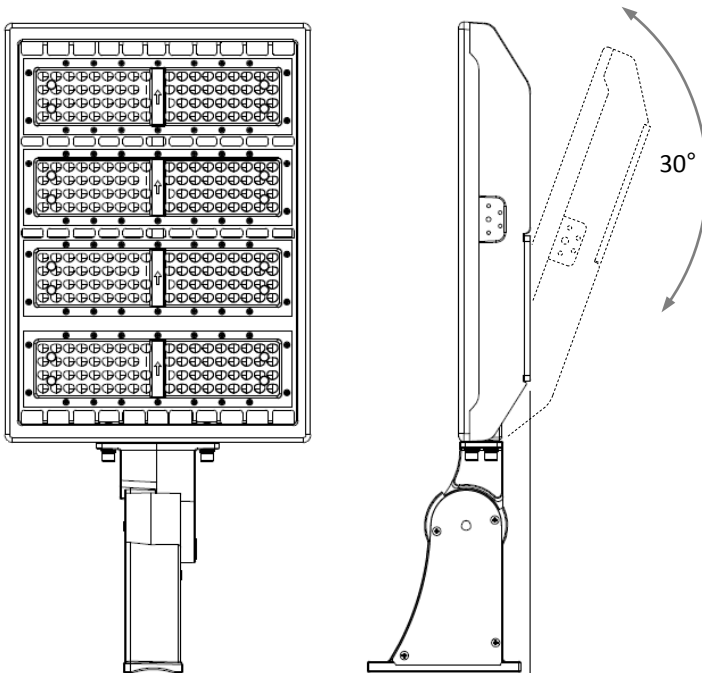
Adjustable Arm Mount LEDMPALPRO-ARM
