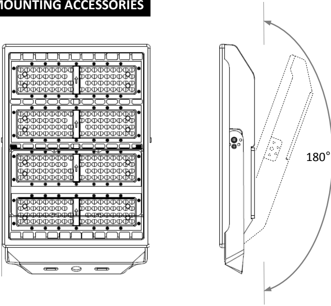
Yoke Mount LEDMPALPRO-YK-S
