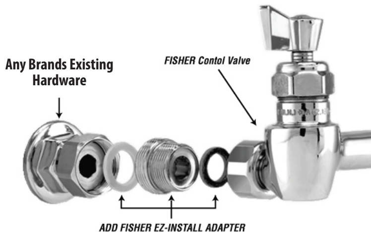
STEP 3 - Place new washer into fitting. Thread in FISHER EZ-Install Adapter.
